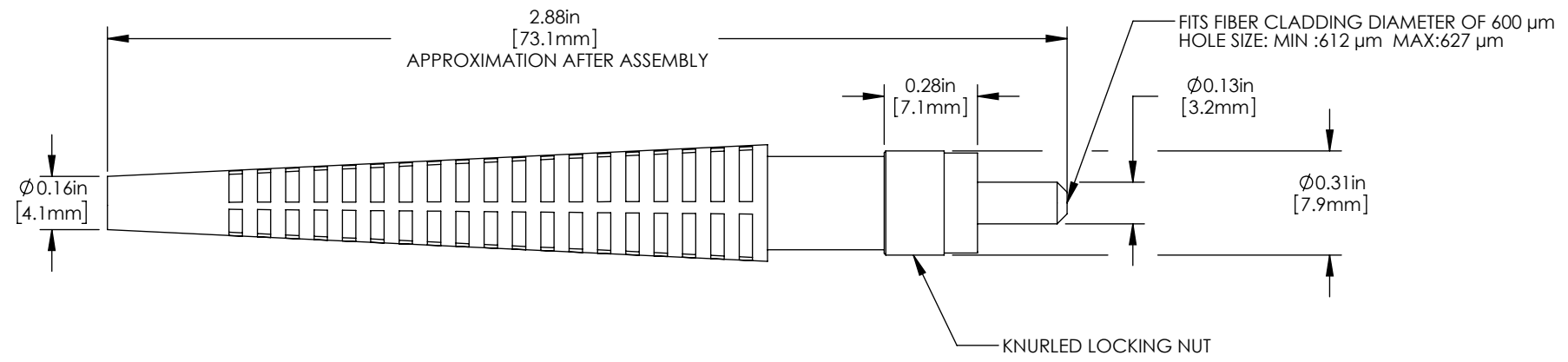
ASSEMBLED VIEW
