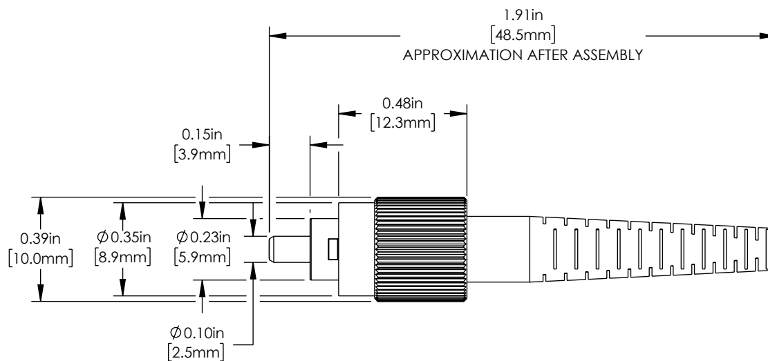
ASSEMBLED VIEW
