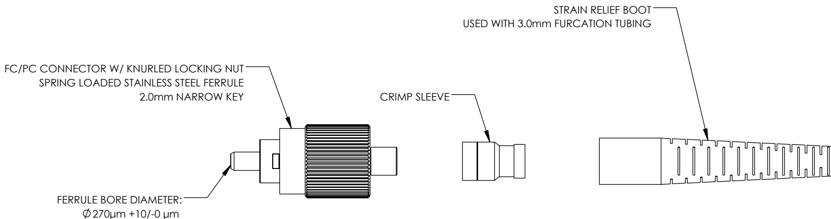
EXPLODED VIEW
