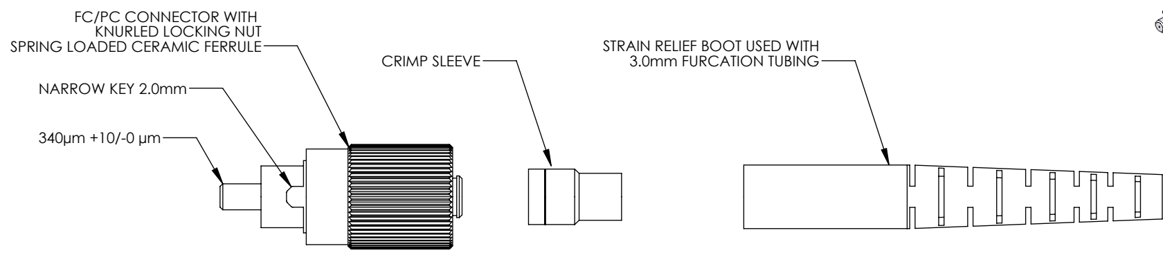
EXPLODED VIEW
