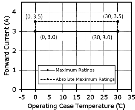
Figure 1. Derating Characteristics
