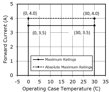
Figure 1. Derating Characteristics
